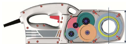
5 Gear Reduction in Aluminum Cast Housing
